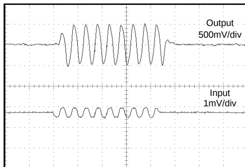
PULSE RESPONSE (BURSTS) (Differential, V_{\text{CA\_CNTL}} = 3.0\text{V} , \text{MGS} = 111 )
