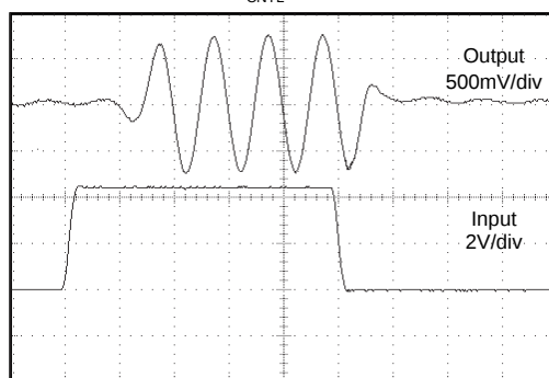
GAIN RESPONSE (Differential, V_{\text{CA\_CNTL}} Pulsed, \text{MGS} = 111 )
