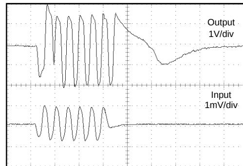
OVERLOAD RECOVERY (Differential, V_{\text{CA\_CNTL}} = 3.0\text{V} , \text{MGS} = 111 )
