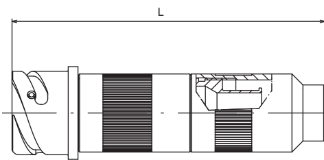
VBN3SS Straight backshell with shielding system VBN3RSS Same as "SS" but includes a wire sealing grommet
