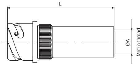
VBN3AM Straight backshell with metric thread and without accessories VBN3RM Same as "AM" but includes a wire sealing grommet
