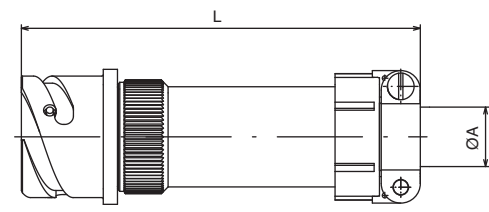
VBN3AF Straight backshell with "A" style clamp VBN3F Same as "AF" but includes a wire sealing grommet
