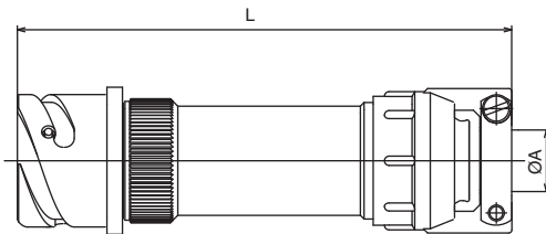
VBN3CF Straight backshell with "C" style clamp VBN3CFZ Same as "CF" but includes a wire sealing grommet
