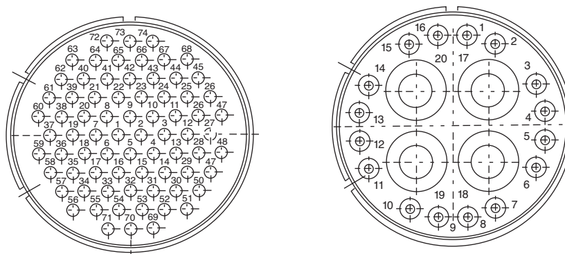
CONTACTS ARRANGEMENTS
