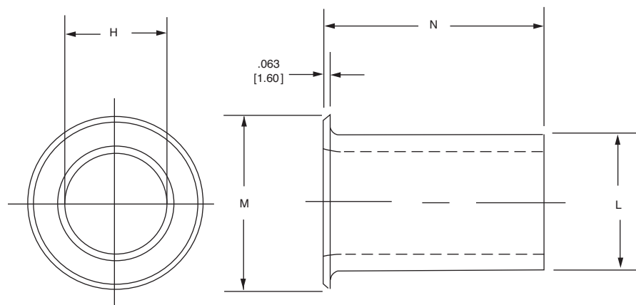
Rubber Bushing
