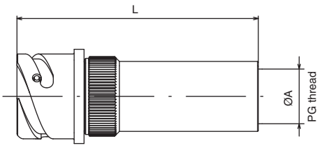
VBN3APG Straight backshell with "PG" thread and without accessories VBN3RPG Same as "APG" but includes a wire sealing grommet
