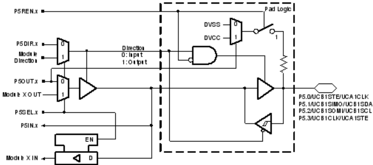
Port P5.0 to P5.3 pin functions
