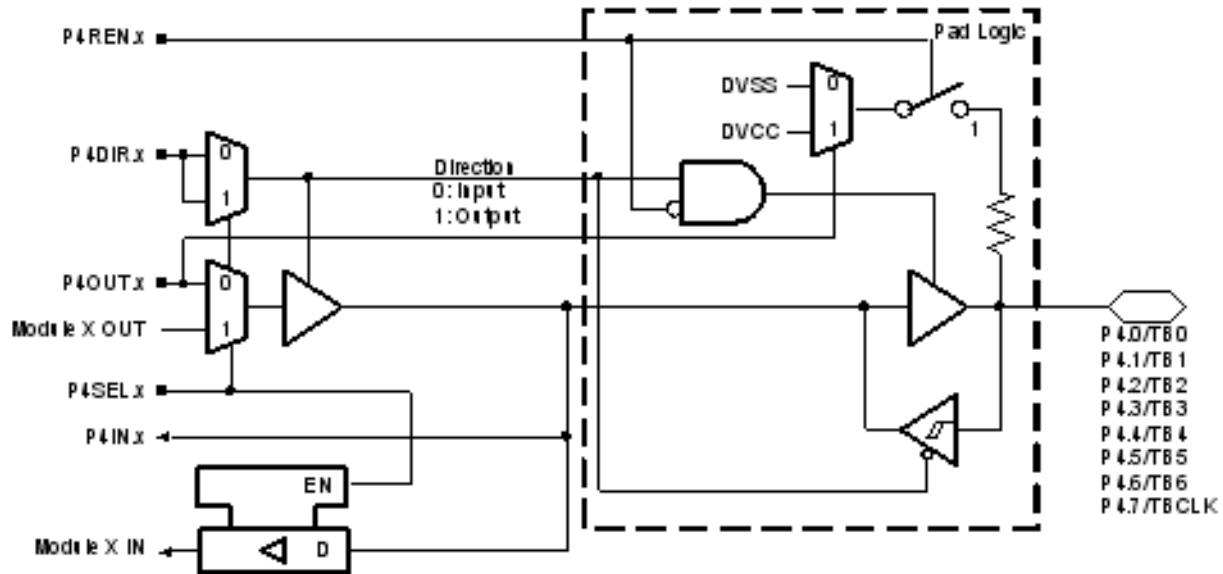
Port P4.0 to P4.7 pin functions
