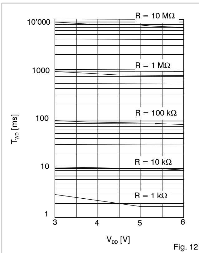
T_{WD} versus V_{DD} at T_A = +25 °C
