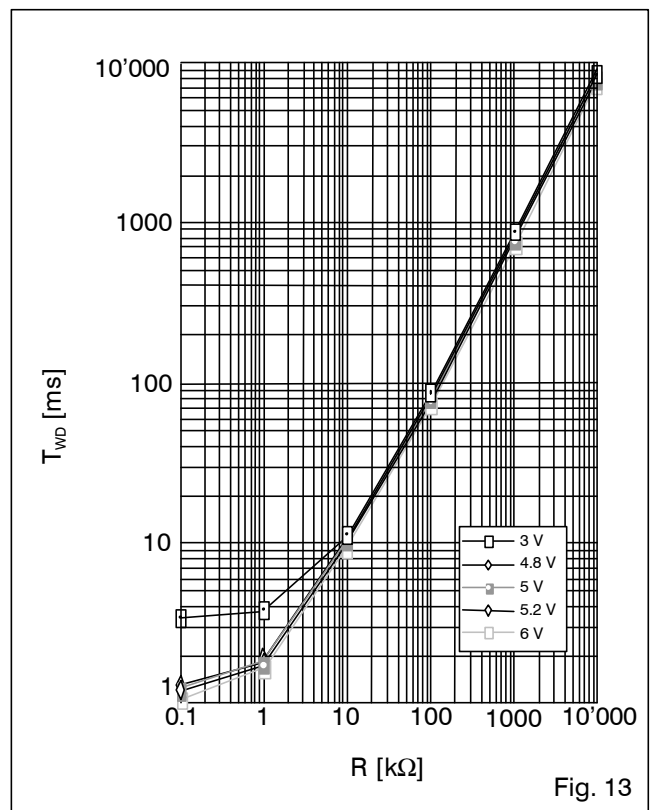
T_{WD} versus R at T_A = +25 °C
