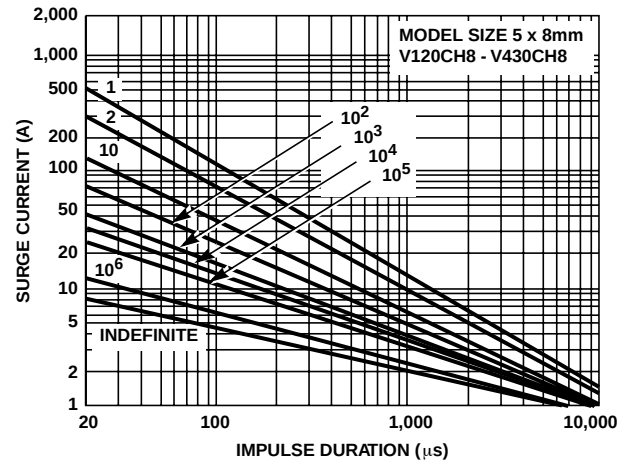
FIGURE 6. SURGE CURRENT RATING CURVES FOR V120CH8 - V430CH8
