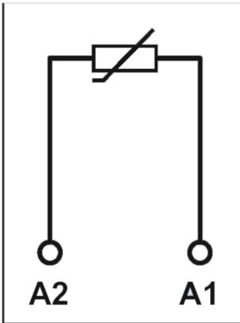
Circuit diagram
