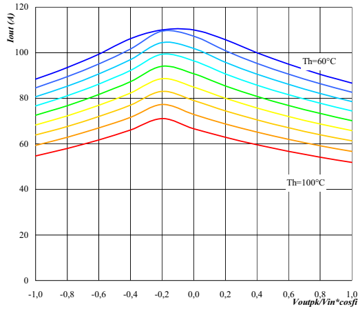
Figure 5. Typical available 50Hz output current as a function of V_{outpk}/V_{in} \cdot \cos\phi Phase I_{out} = f(M_i \cdot \cos\phi_i)
