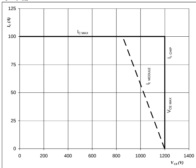
Figure 29 IGBT Reverse bias safe operating area
