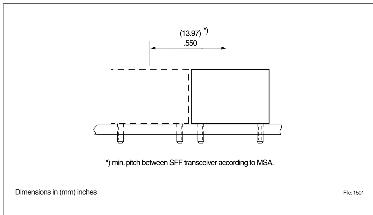
Figure 10 Transceiver Pitch
