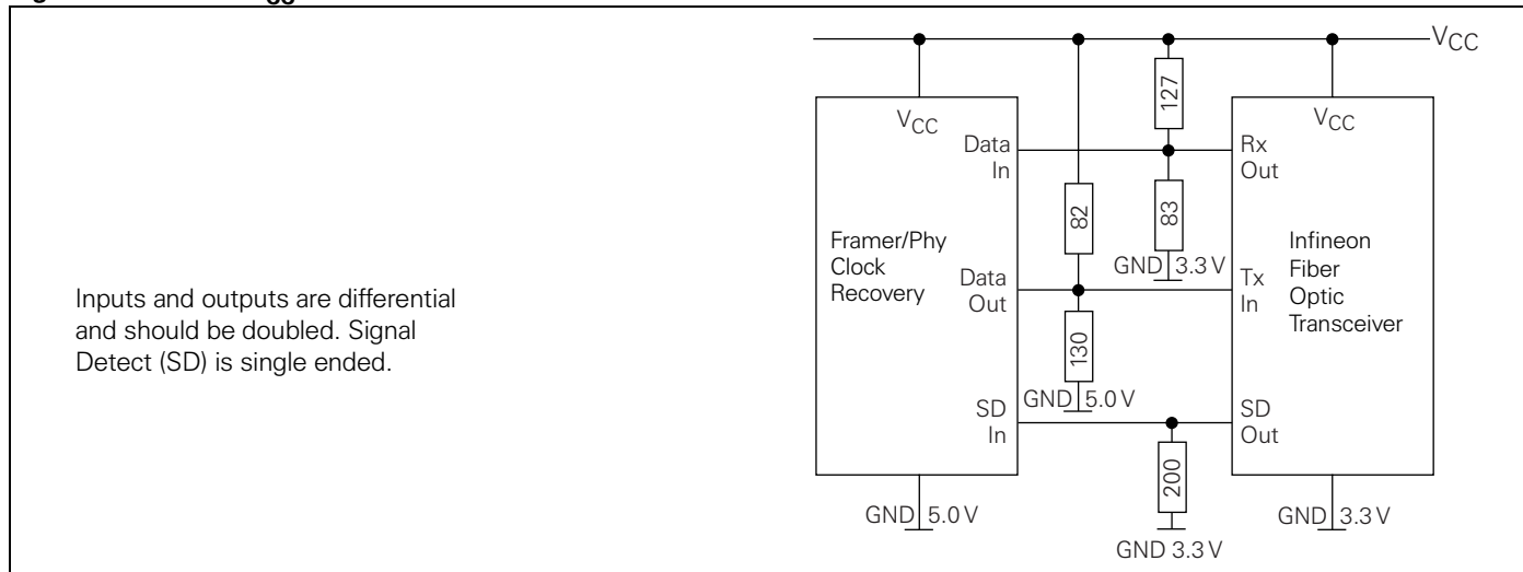
Figure 2. Common V CC
