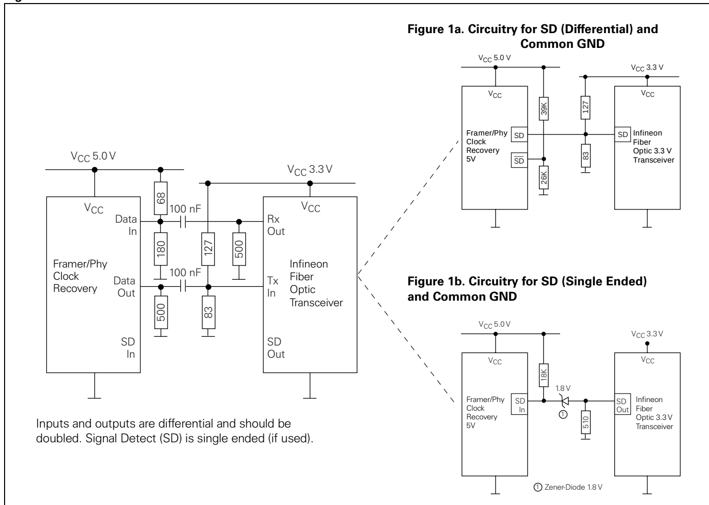
Figure 1. Common GND
