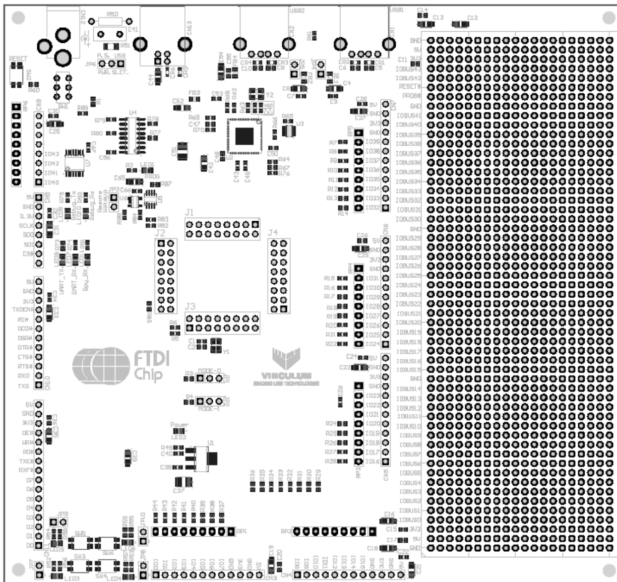
Figure 3.1 V2-EVAL Board Layout
