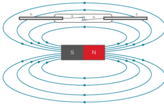
Figure 3.1. Reed Switch
