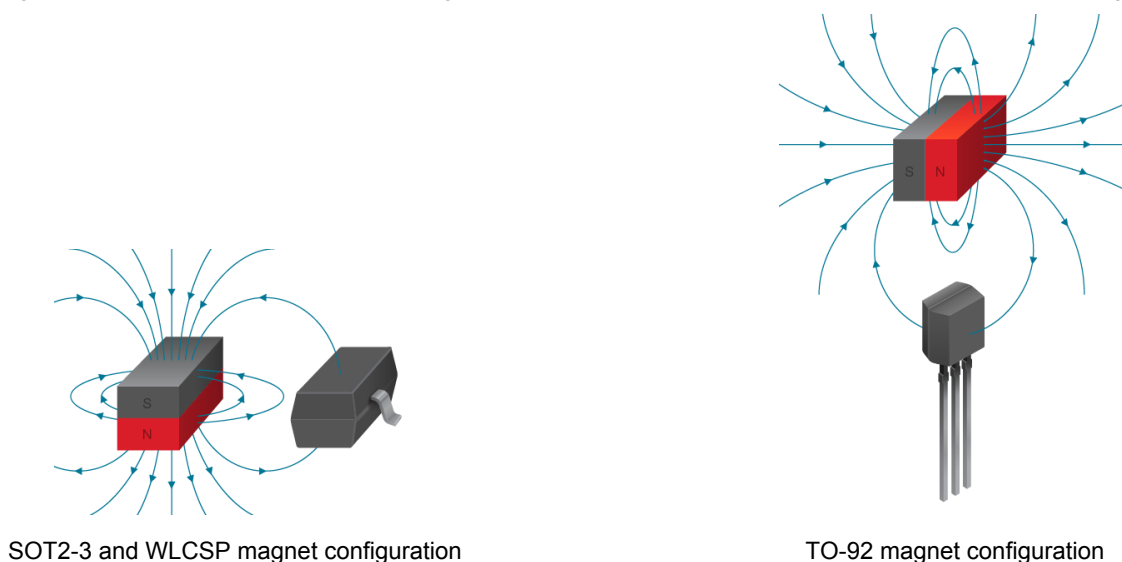
Figure 3.4. SOT23, DFN-8 and TO-92 Magnet Configuration
