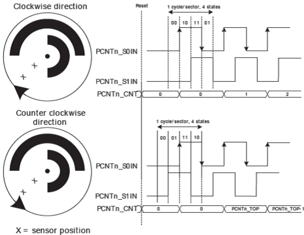
Figure 10.1. Low-Power Quadrature Decoding Logic
