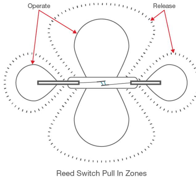
Figure 3.2. Reed Switch Pull-In Zones
