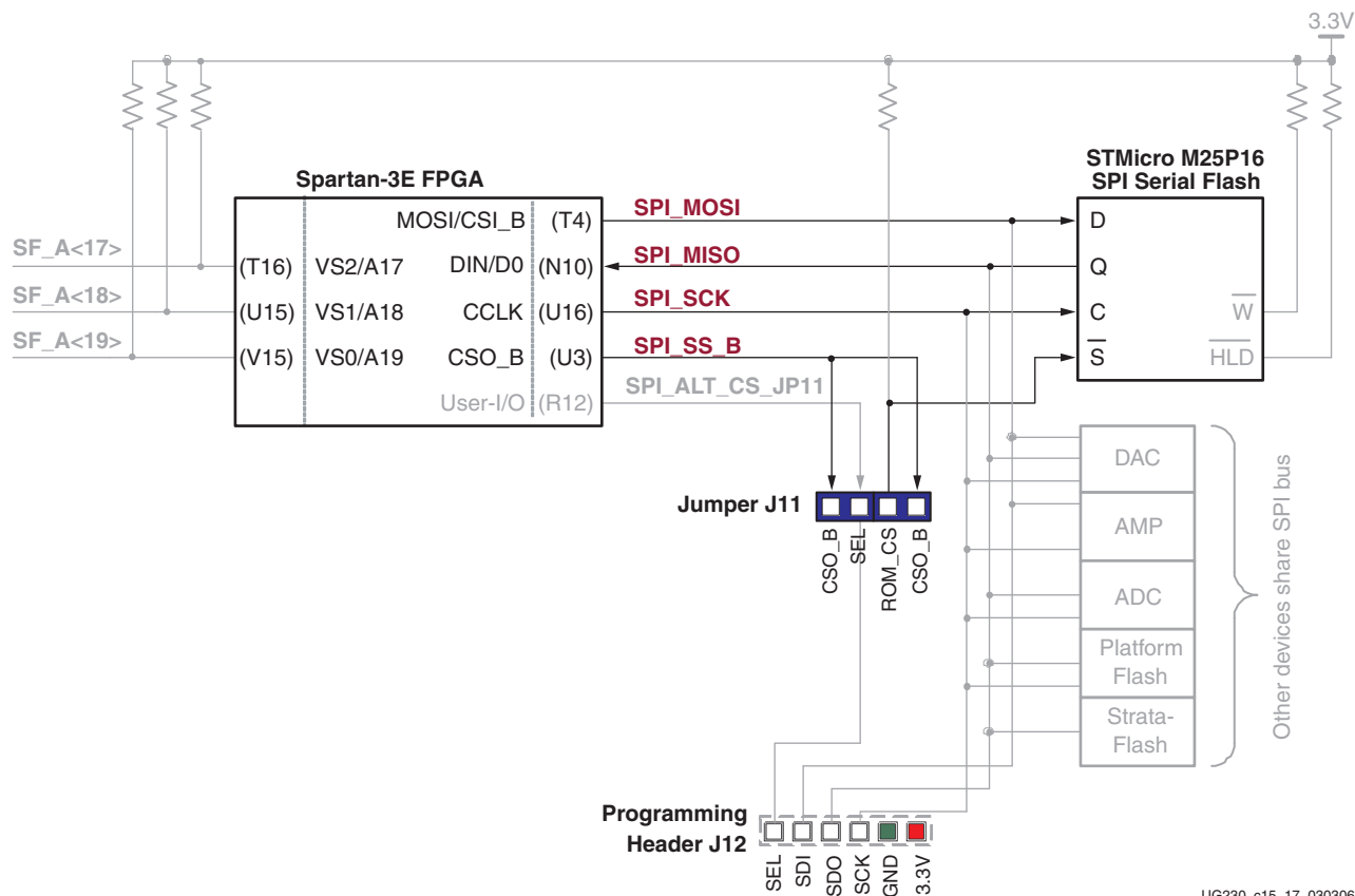
Figure 12-17: Additional SPI Flash Interface Design Details
