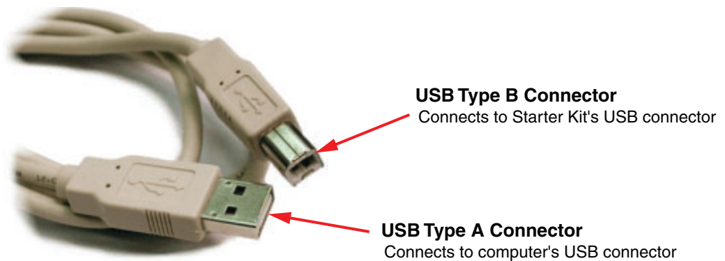
Figure 4-3: Standard USB Type A/Type B Cable
