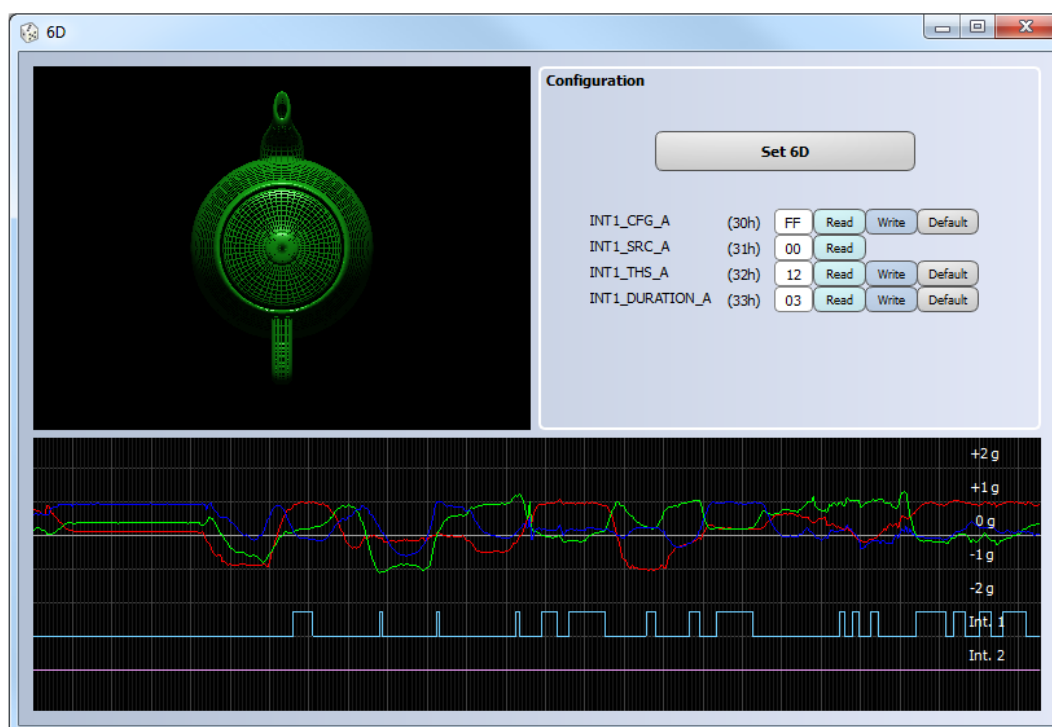
Figure 20. 6D tool
