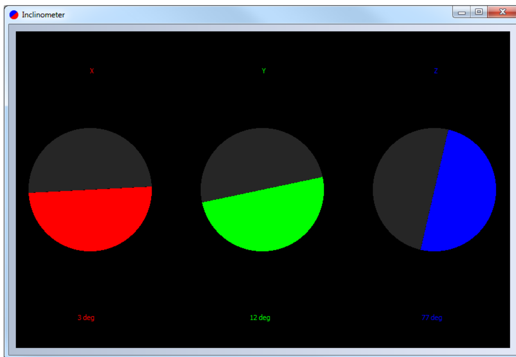
Figure 19. Inclinometer tool
