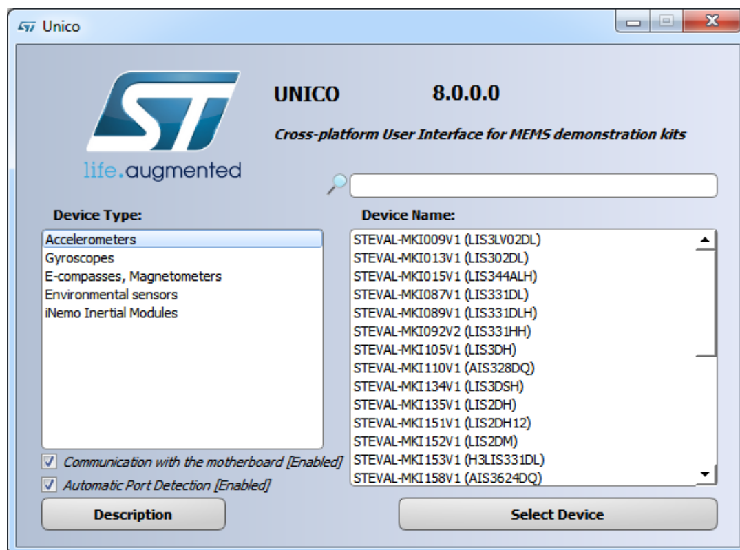
Figure 1. Unico launcher
