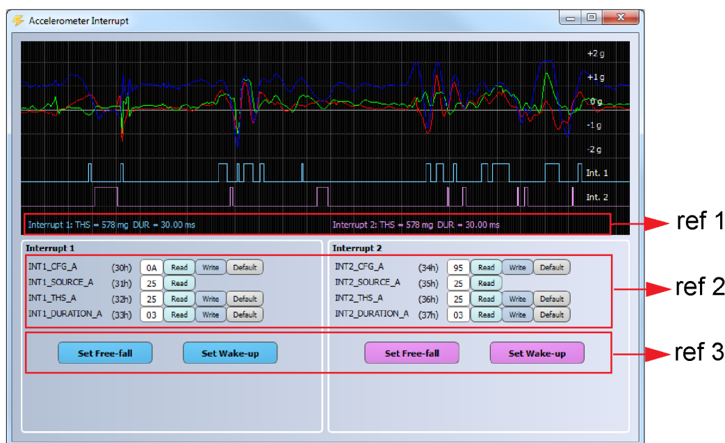
Figure 10. Interrupt tool
