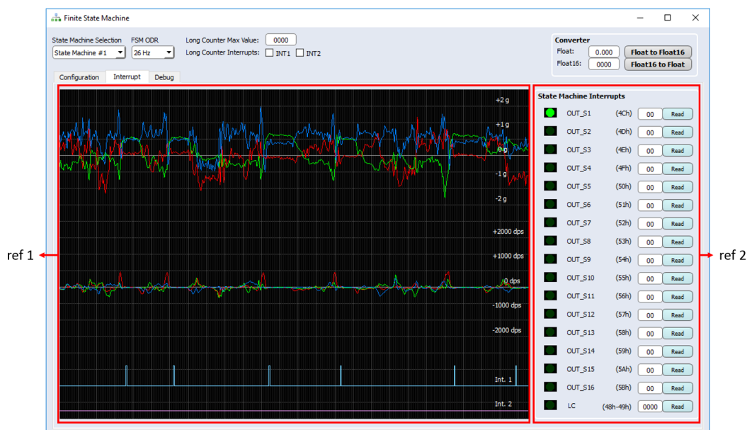
Figure 14. Interrupt tab
