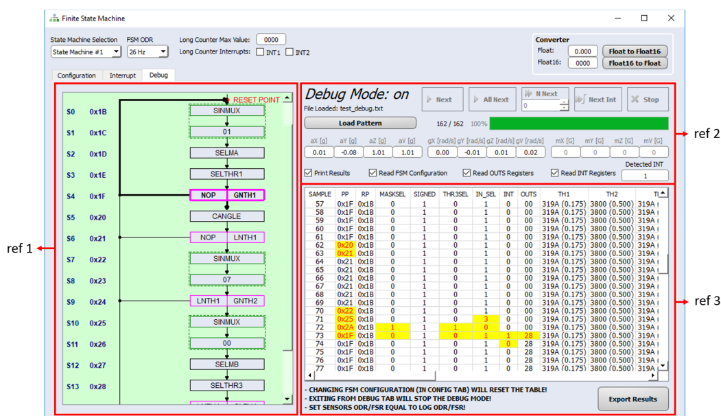
Figure 15. Debug tab
