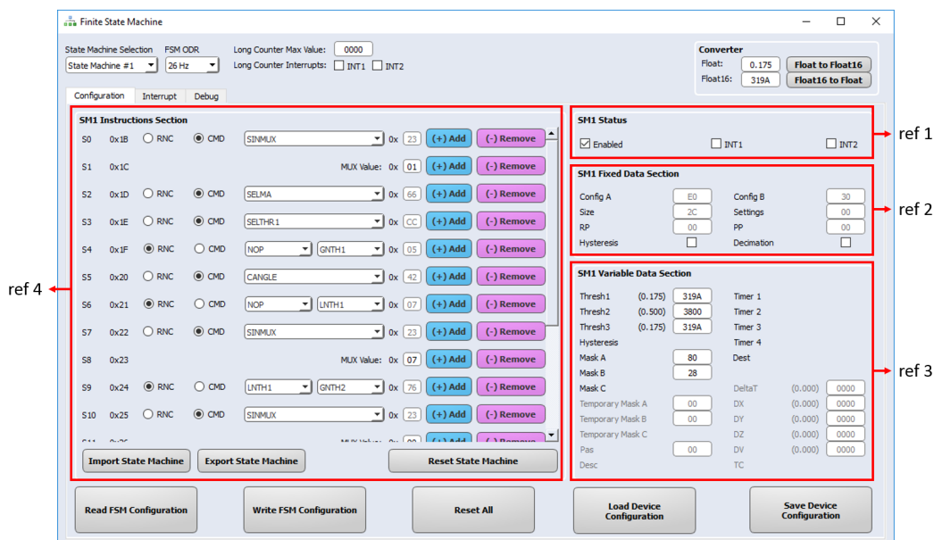
Figure 13. Configuration tab
