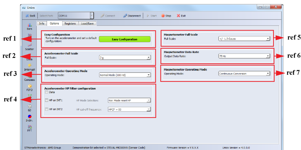
Figure 3. Options tab
