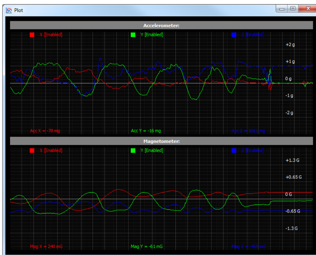
Figure 7. Plot tool
