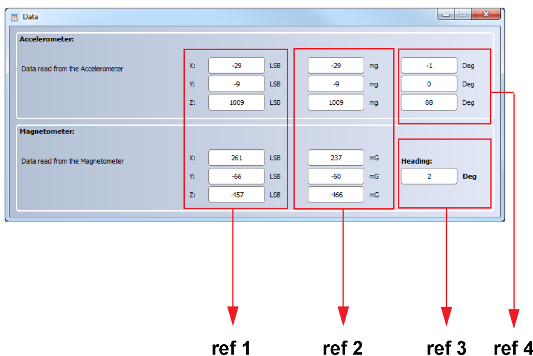
Figure 9. Data tool
