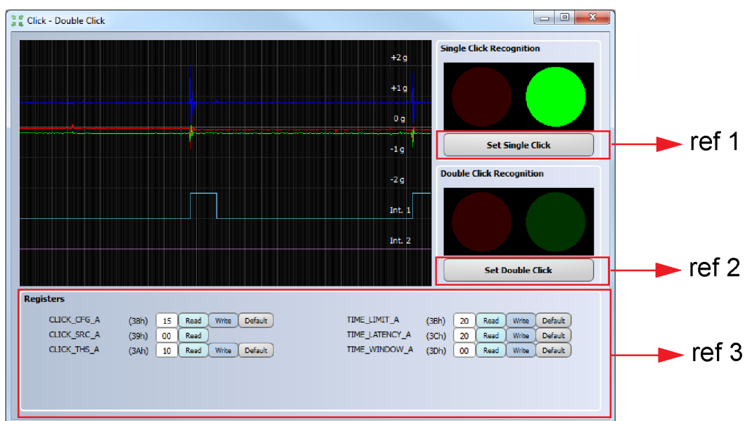
Figure 18. Click tool
