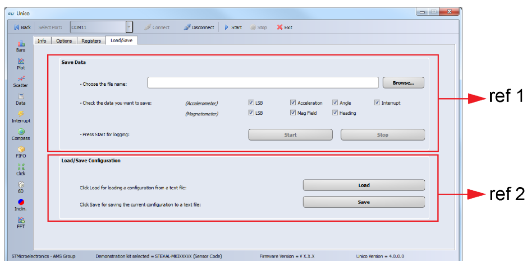
Figure 5. Load/Save tab
