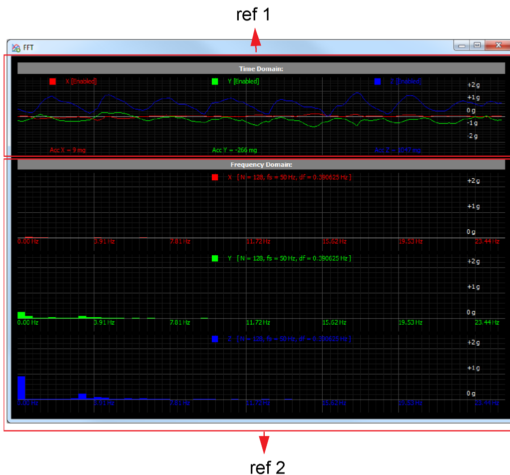
Figure 21. FFT tool
