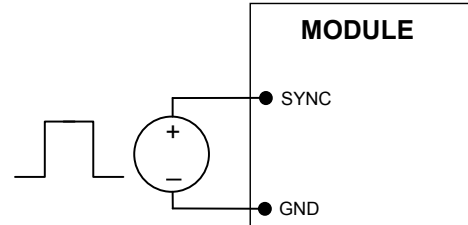
Figure 6. External source connections to synchronize switching frequency of the module.
