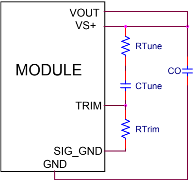
Figure. 7. Circuit diagram showing connection of R_{TUNE} and C_{TUNE} to tune the control loop of the module.
