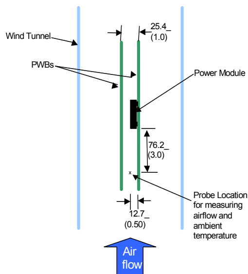
Figure 8. Thermal Test Setup.
