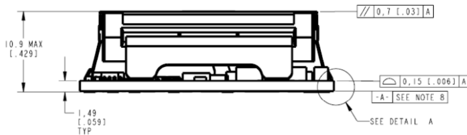
SIDE VIEW
