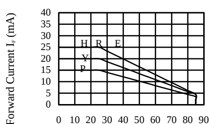
FIG.3 ALLOWABLE DC CURRENT VS. AMBIENT TEMPERATURE
