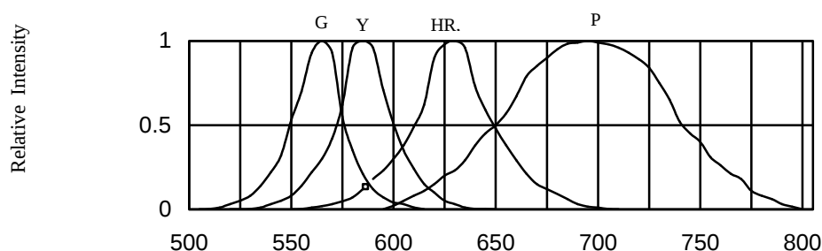
FIG.1 RELATIVE LUMINOUS INTENSITY VS. WAVELENGTH
