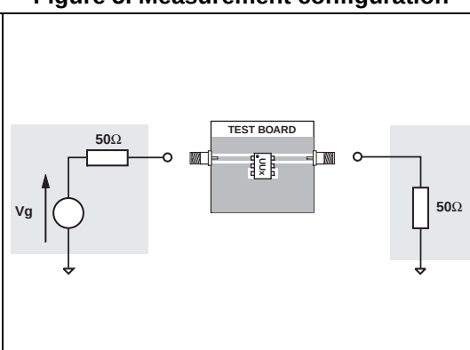
Figure 5. Measurement configuration
