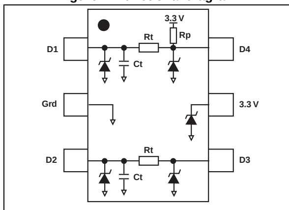
Figure 1. Functional diagram
