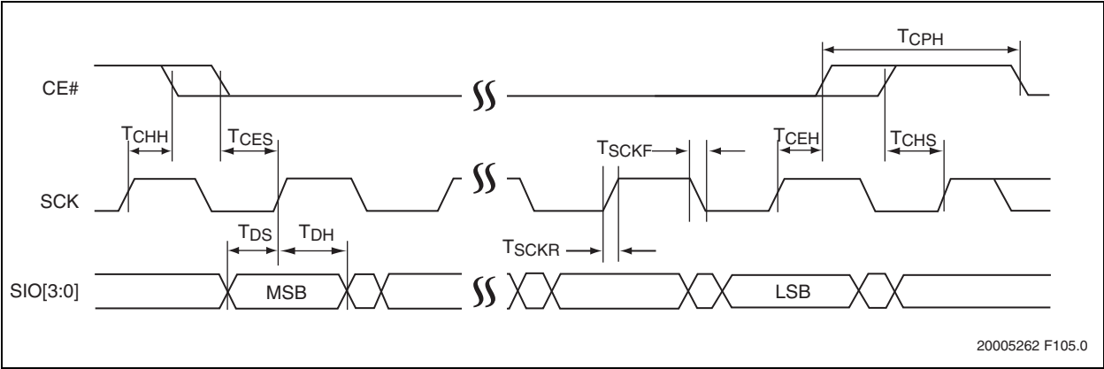
FIGURE 7-2: SERIAL INPUT TIMING DIAGRAM
