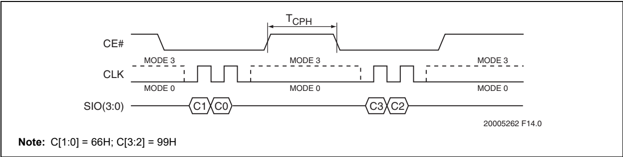
FIGURE 7-4: RESET TIMING DIAGRAM
