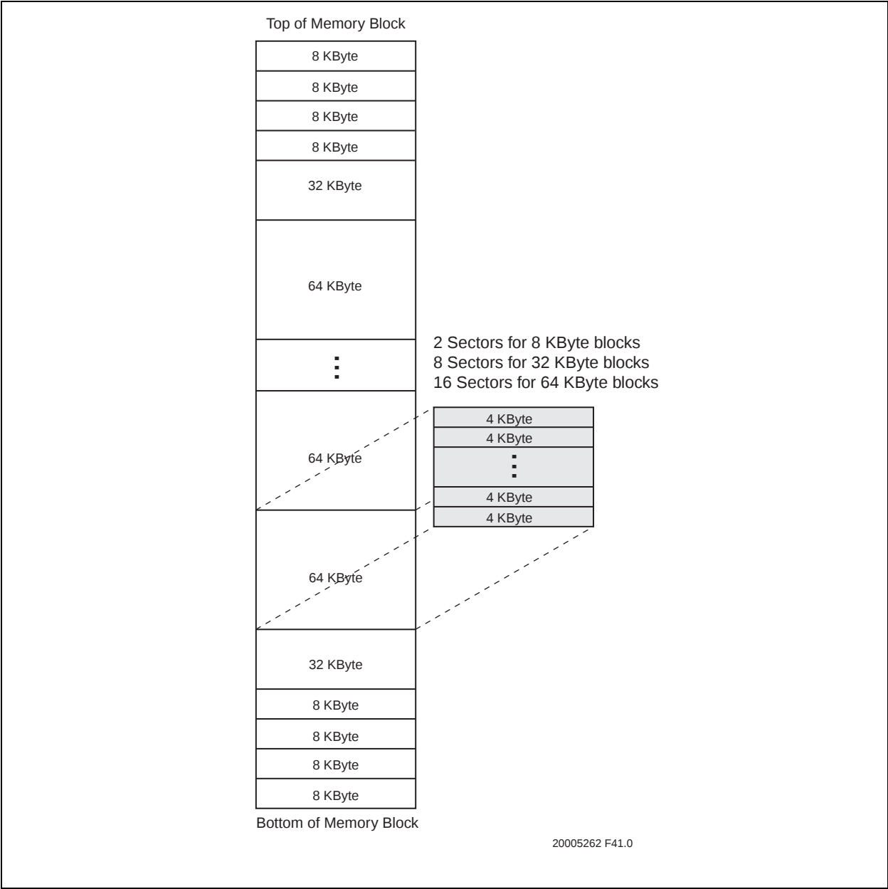
FIGURE 2-1: MEMORY MAP
