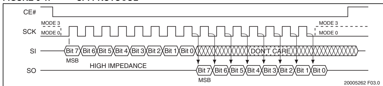
FIGURE 3-1: SPI PROTOCOL
