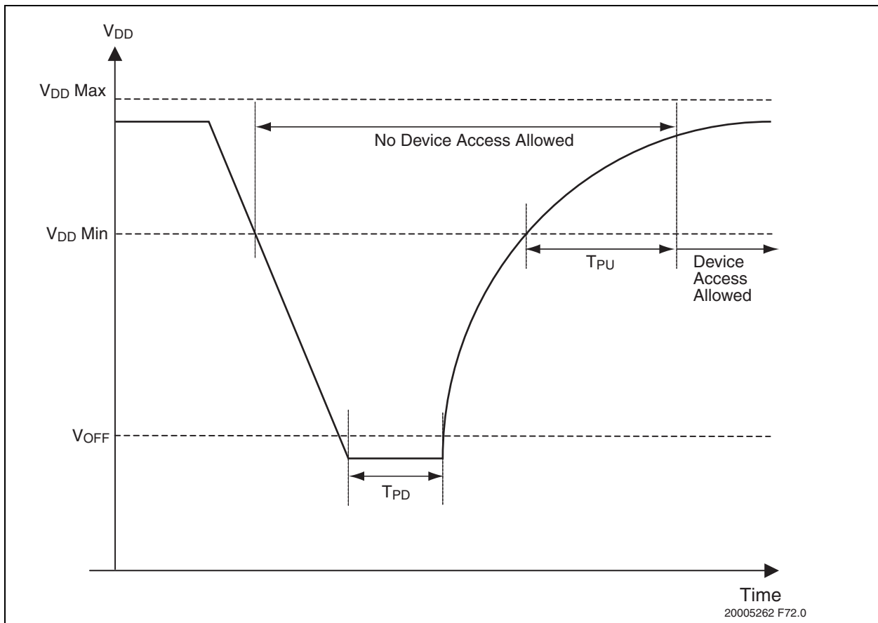
FIGURE 5-2: POWER-DOWN AND VOLTAGE DROP DIAGRAM
