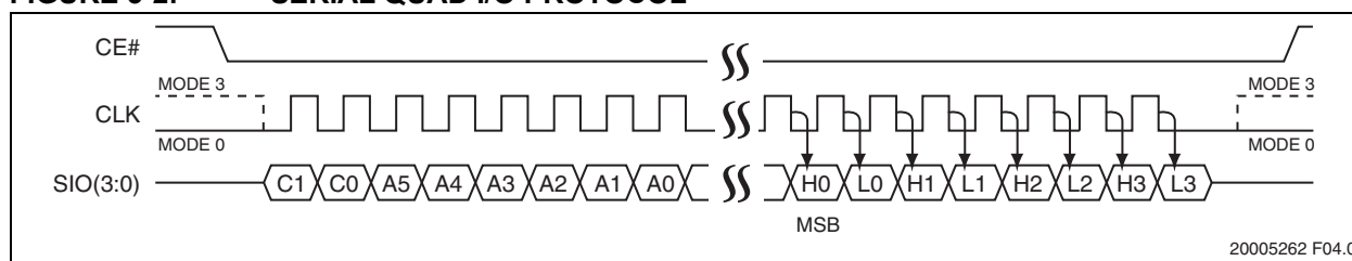
FIGURE 3-2: SERIAL QUAD I/O PROTOCOL
