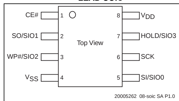
FIGURE 1-2: PIN DESCRIPTION FOR 8-LEAD SOIC
