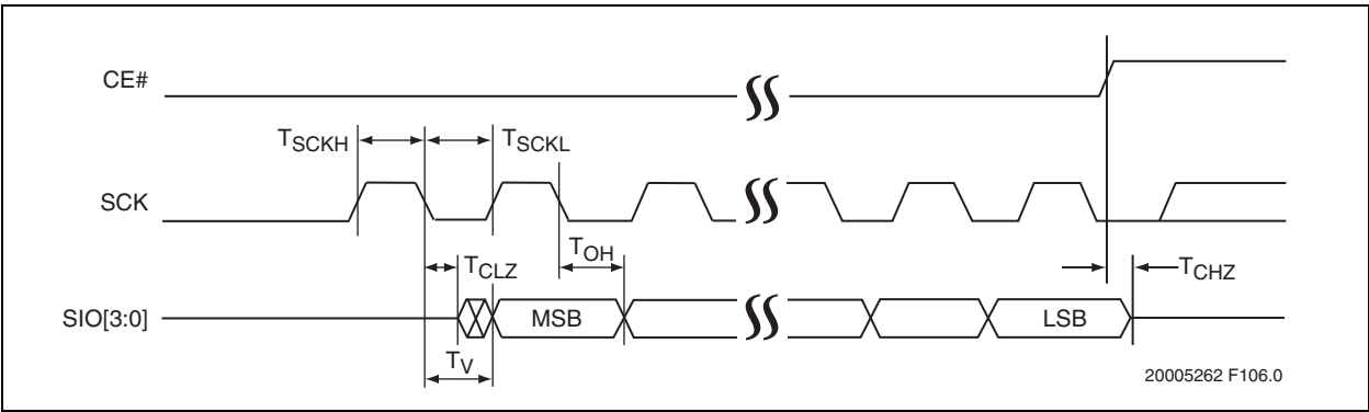
FIGURE 7-3: SERIAL OUTPUT TIMING DIAGRAM
