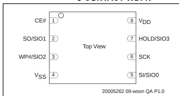
FIGURE 1-1: PIN DESCRIPTION FOR 8-CONTACT WDFN
