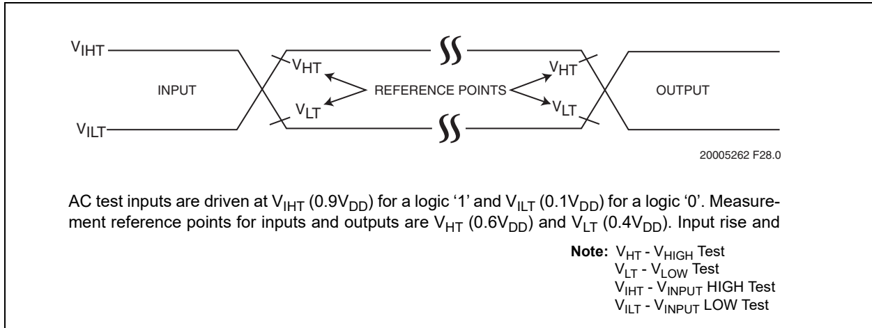
FIGURE 7-5: AC INPUT/OUTPUT REFERENCE WAVEFORMS
