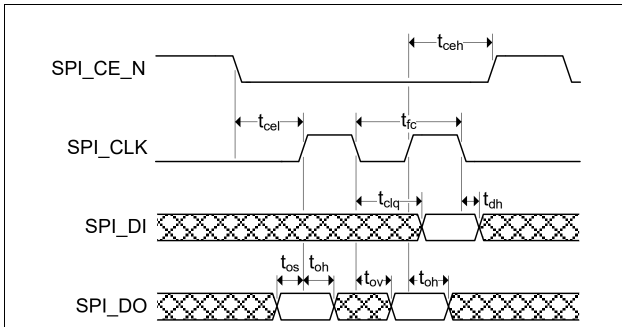
FIGURE 9-4: SPI TIMING
