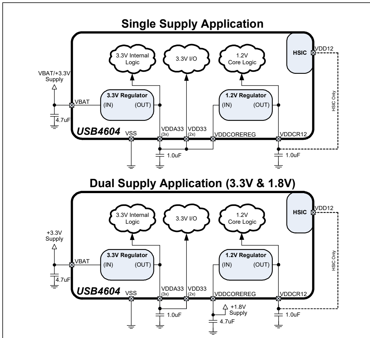
FIGURE 4-1: POWER CONNECTIONS
