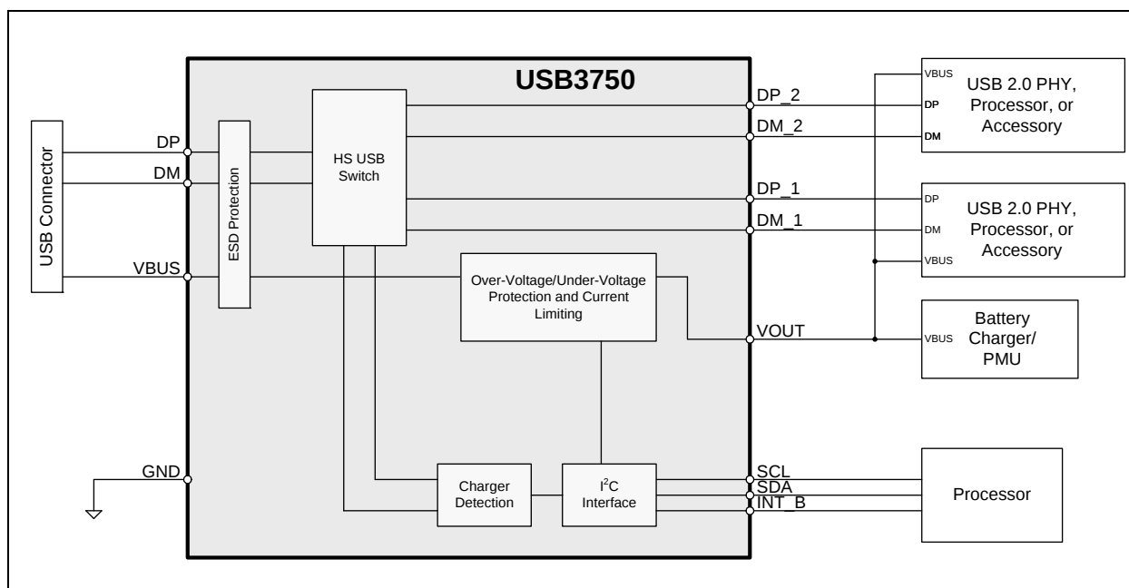
FIGURE 4-1: USB3750 BLOCK DIAGRAM
