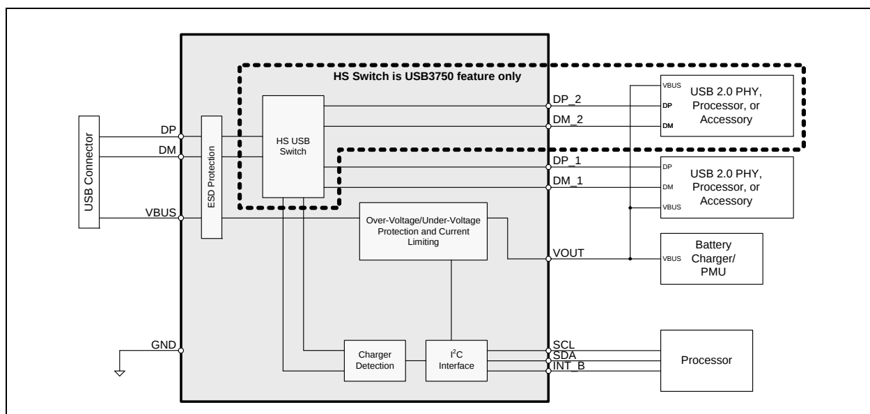
USB375x Block Diagram
