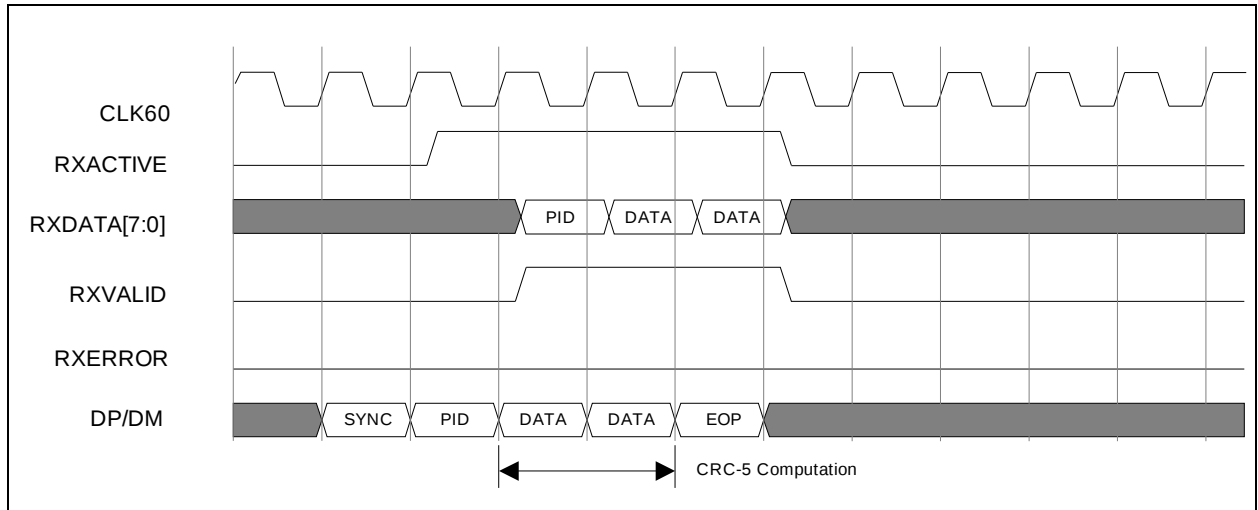
FIGURE 7-11: RECEIVE TIMING FOR SETUP PACKET (8-BIT MODE)
