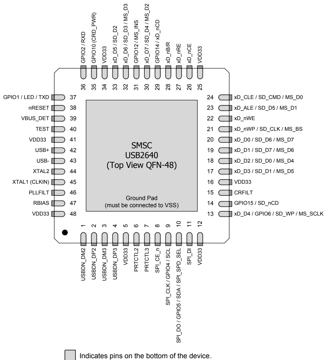
Figure 3.1 USB2640 48-Pin QFN
