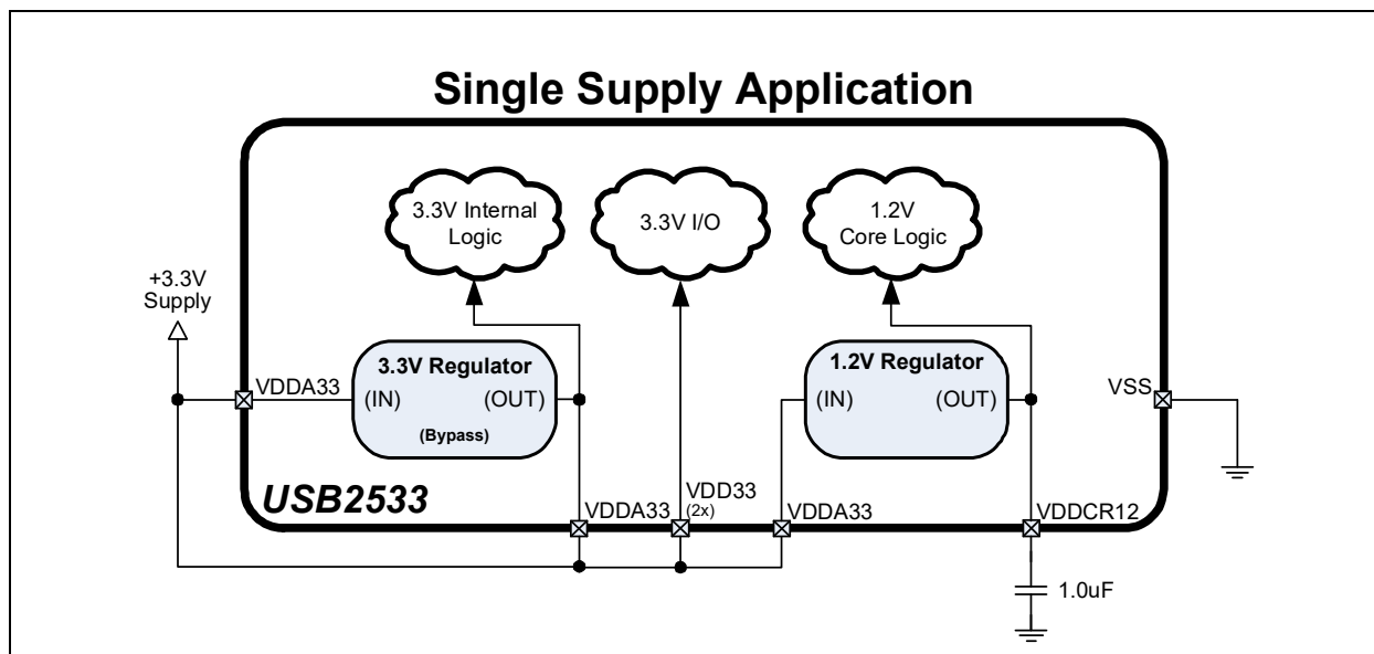
FIGURE 4-1: POWER CONNECTIONS
