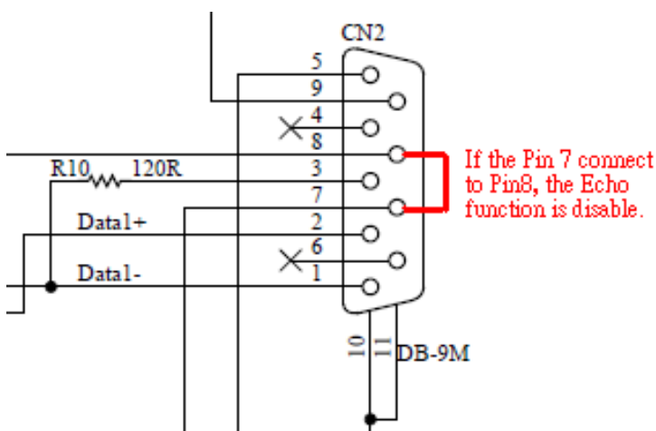
Figure 2.1 USB-COM485-PLUS2 Termination resistor and echo disable
