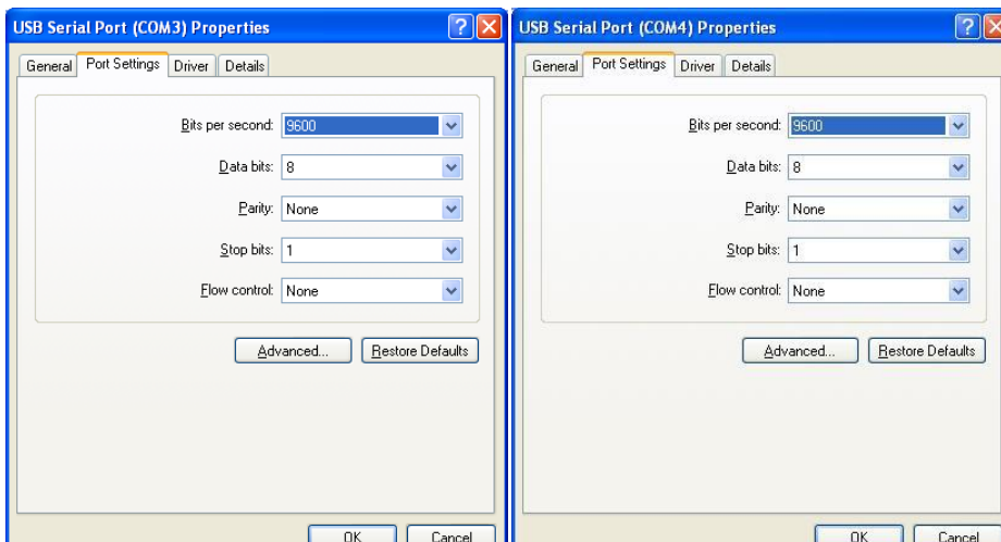
Figure 2.9 - Settings Tab
