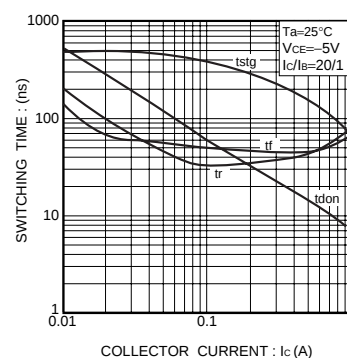
Fig.6 Switching time
