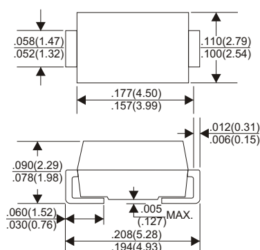
DO-214AC
