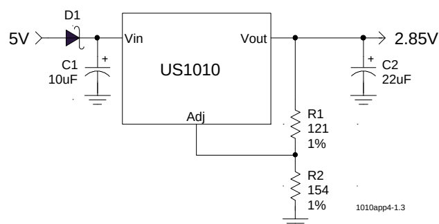
Figure 4 - Final Schematic for half of the GTL+ termination regulator.
