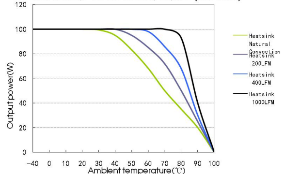
URF1D15QB-100WH Thermal Curves (Vin=110V)
