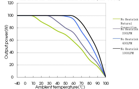
URF1D24QB-100W Thermal Curves (Vin=110V)
