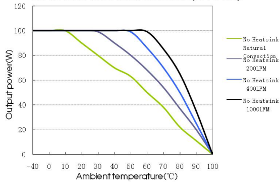
URF1D12QB-100W Thermal Curves (Vin=110V)
