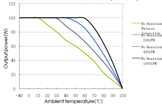
URF1D15QB-100W Thermal Curves (Vin=110V)
