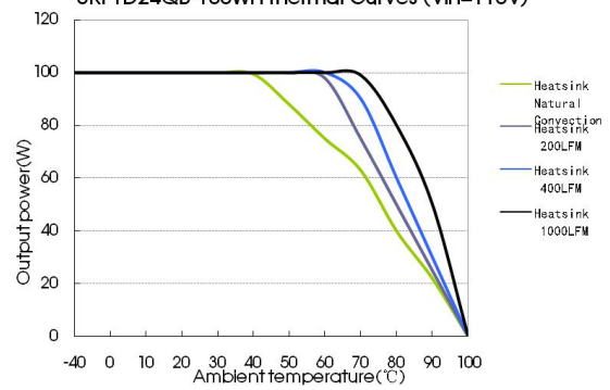
URF1D24QB-100WH Thermal Curves (Vin=110V)
