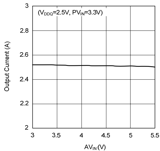
Maximum Sourcing Current vs. AV_{IN}
