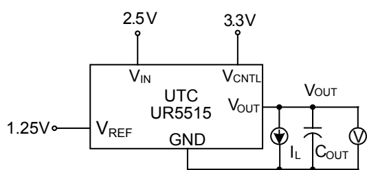
Fig1. Output Voltage Tolerance, V_{OUT}
