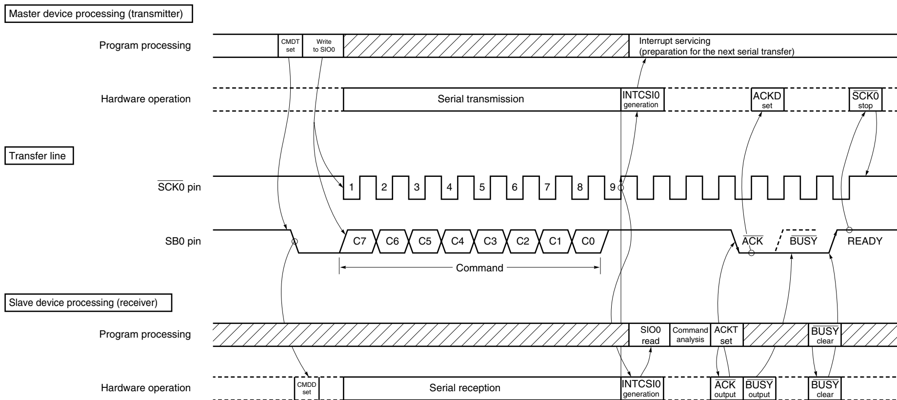
Figure 13-27. Command Transmission from Master Device to Slave Device
