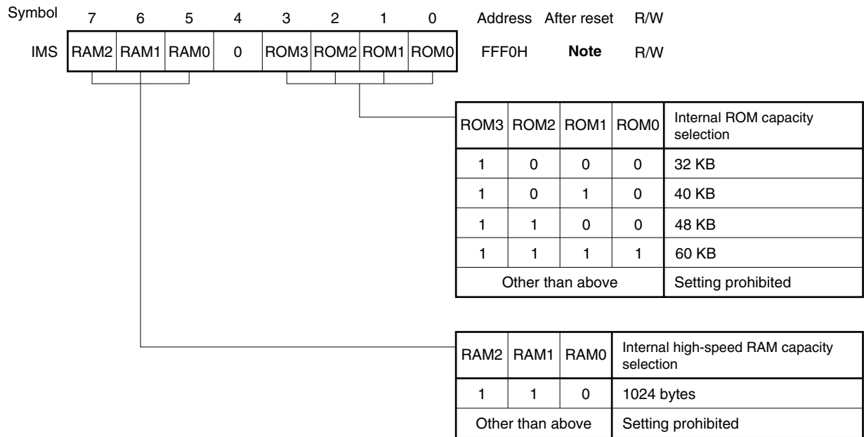
Figure 19-1. Format of Internal Memory Size Switching Register (IMS)
