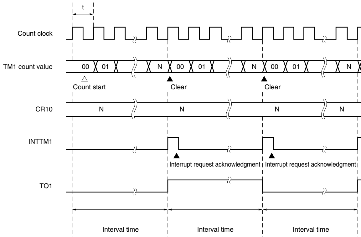
Figure 7-8. Interval Timer Operation Timing
