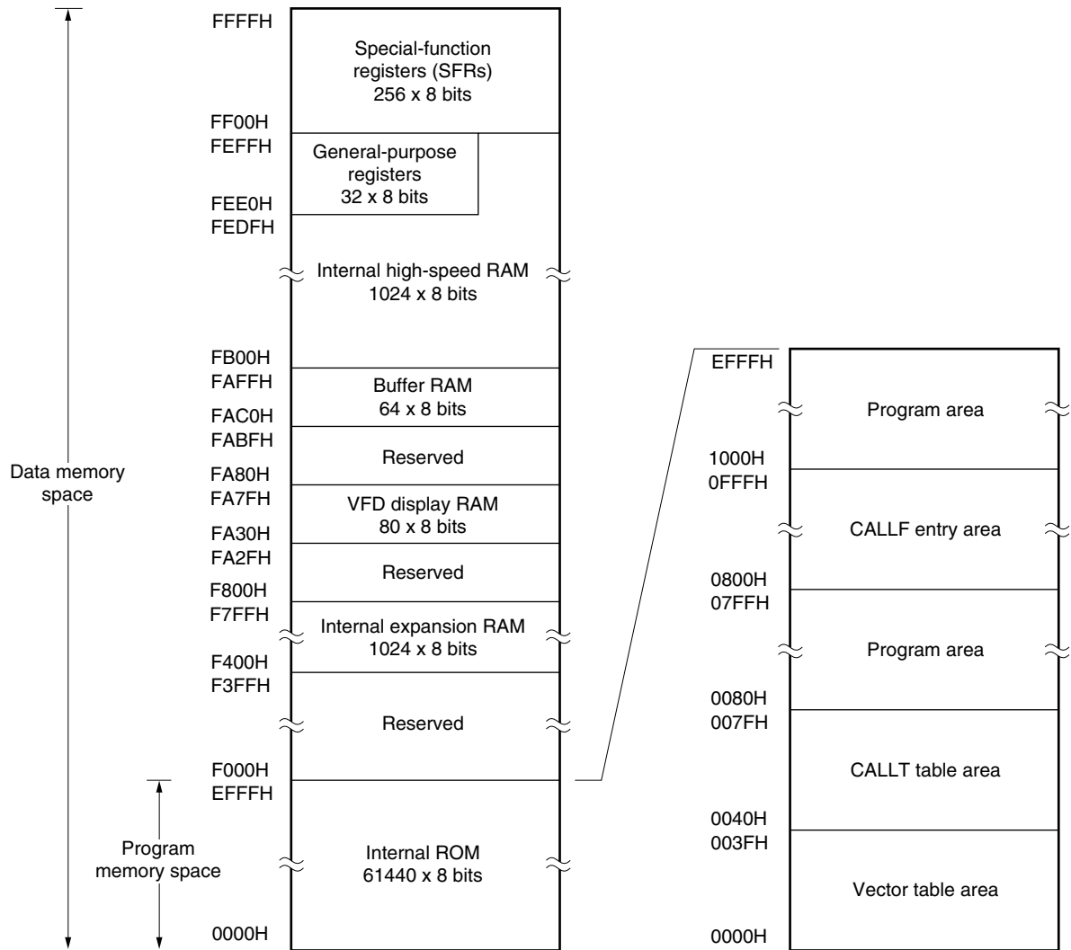
Figure 3-4. Memory Map ( \mu PD780208)
