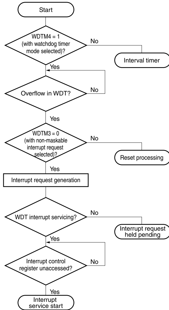
Figure 16-9. Non-Maskable Interrupt Request Acknowledgment Flowchart
