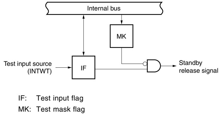
Figure 16-17. Basic Configuration of Test Function
