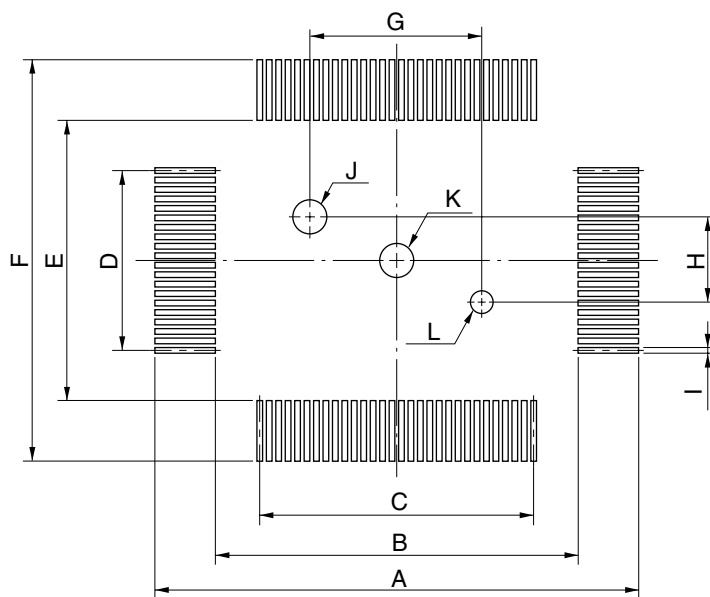
Figure B-3. Recommended Footprint for EV-9200GF-100 (for Reference Purposes only)
