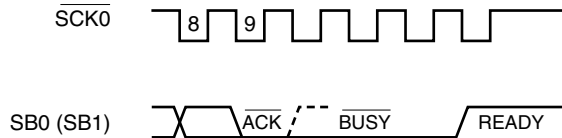
Figure 13-18. \overline{\text{BUSY}} and READY Signals
