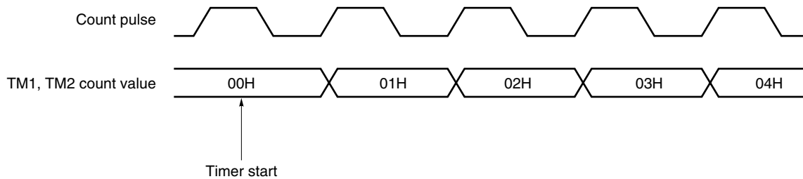
Figure 7-14. 8-Bit Timer Register Start Timing
