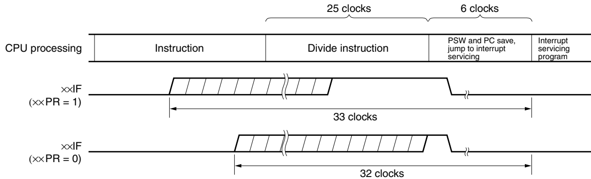
Figure 16-14. Interrupt Request Acknowledgment Timing (Maximum Time)
