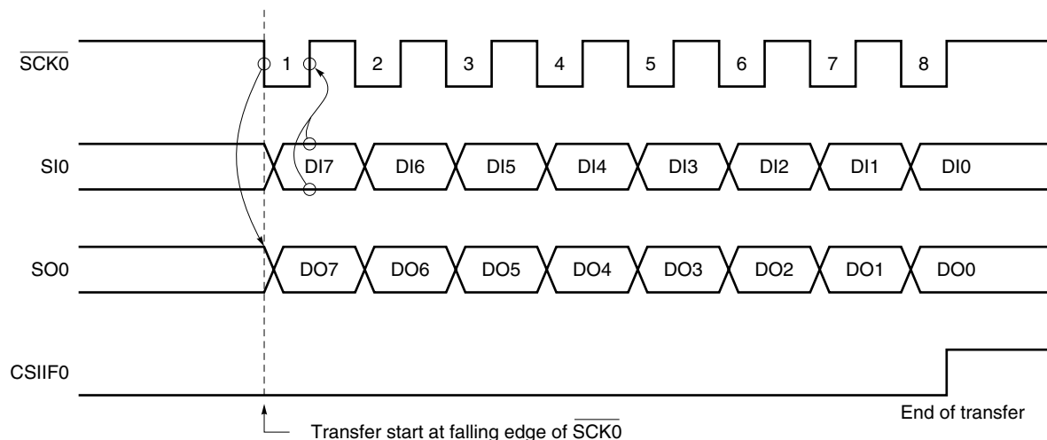
Figure 13-6. 3-Wire Serial I/O Mode Timing
