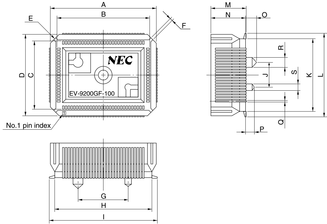
Figure B-2. EV-9200GF-100 Package Drawing (for Reference Purposes only)
