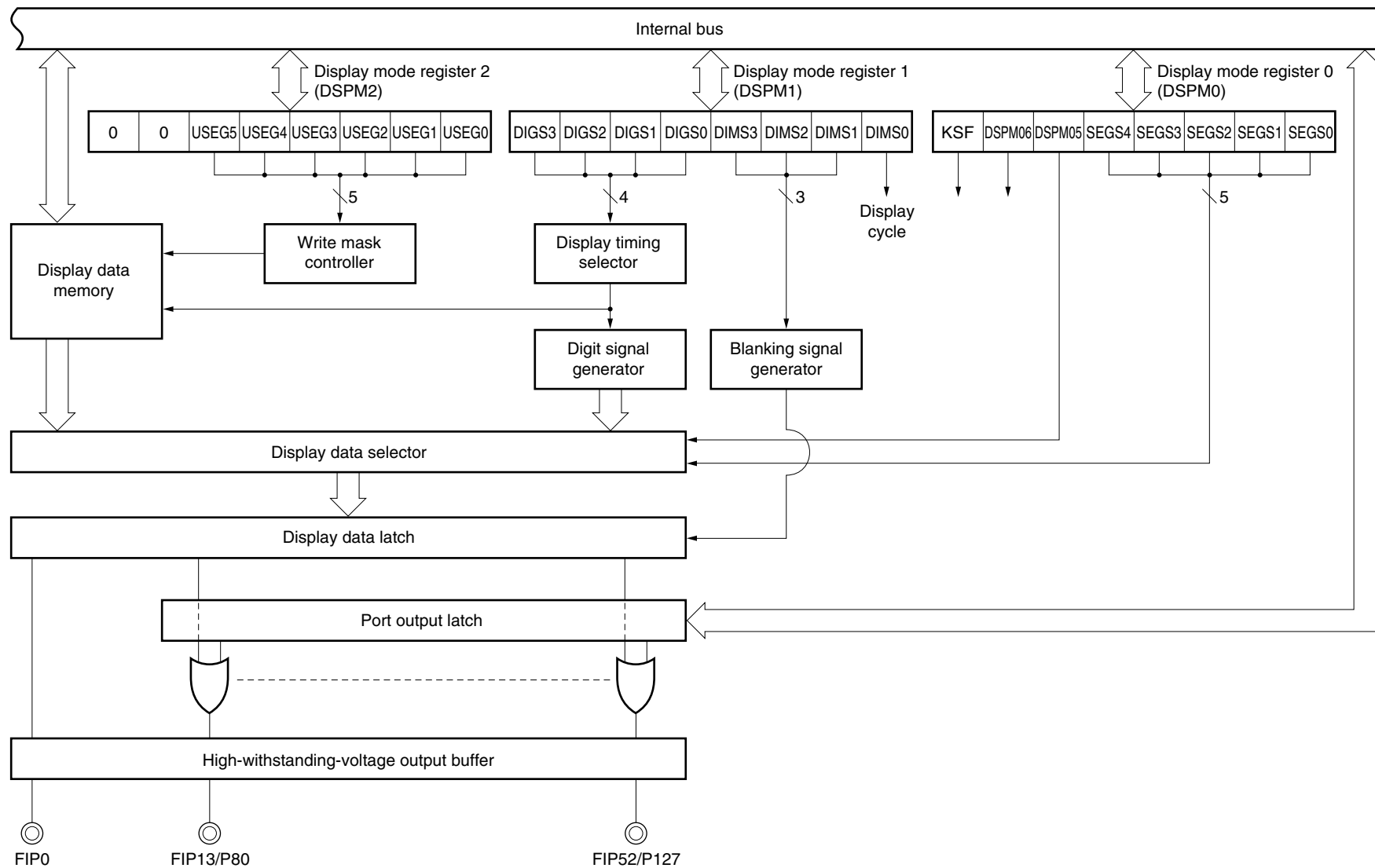
Figure 15-2. VFD Controller/Driver Block Diagram
