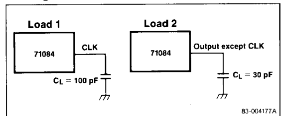
Loading Circuits
