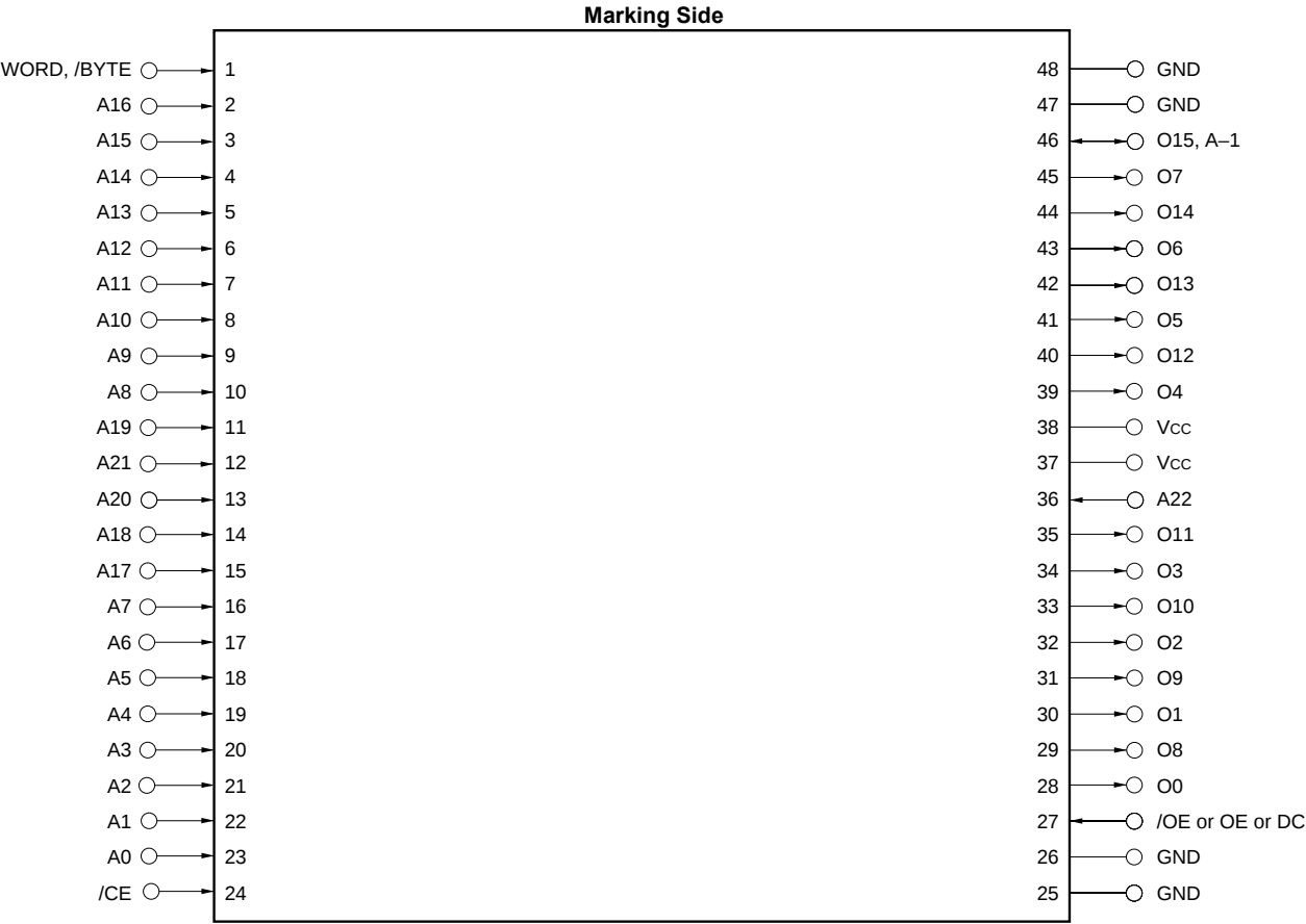
48-pin PLASTIC TSOP(I) (12 x 18) (Normal bent) [ μPD23C128040BLGY-xxx-MJH ] [ μPD23C128080BLGY-xxx-MJH ]
