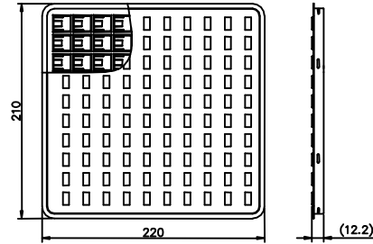
Tray used in UN2E8 / 2H8-XXXL
