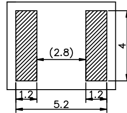
Recommended pad outline
