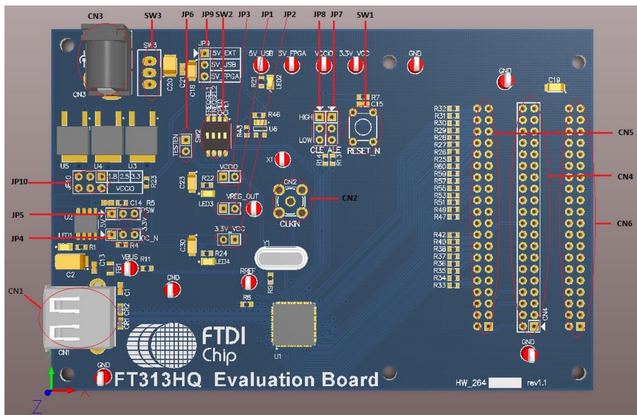
Figure 3.2 – UMFT313EV module top view
