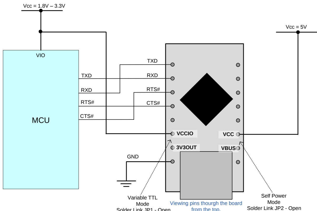
Figure 5.2 – Self-Powered Configuration
