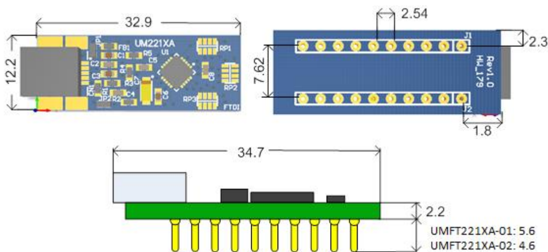
Figure 5.6 – UMFT221XA Module Dimensions
