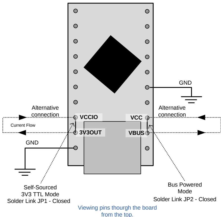
Figure 5.1 – Bus Powered Configuration
