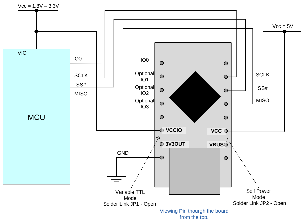
Figure 5.2 – Self-Powered Configuration
