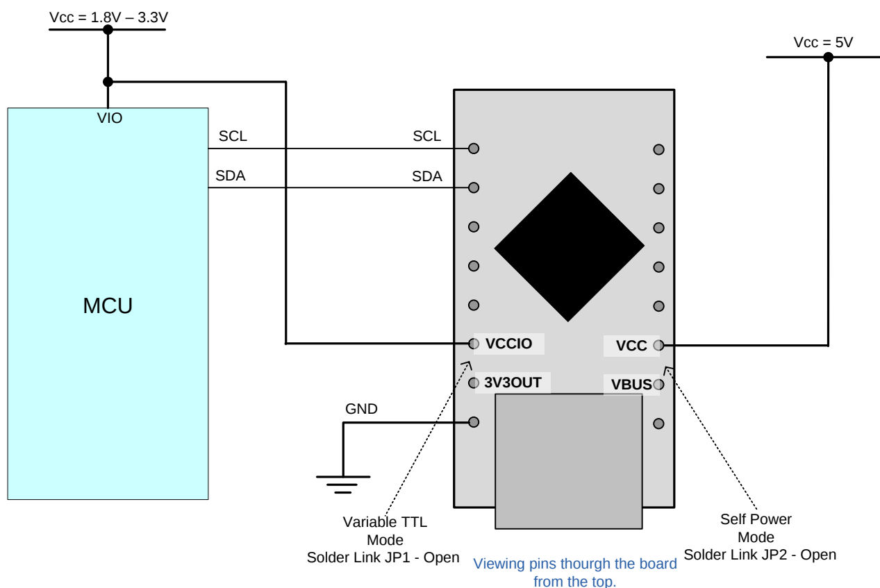
Figure 5.2 – Self-Powered Configuration
