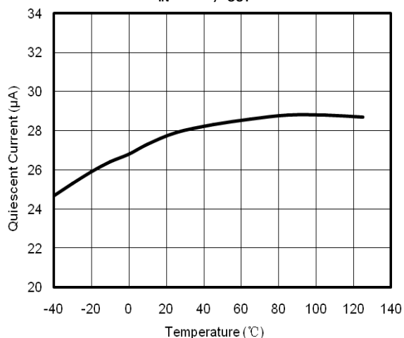
Quiescent Current vs Temperature V_{IN}=2.8V, I_{OUT}=0mA
