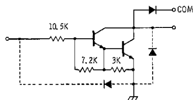
ULS-20X4* (Each Driver)
