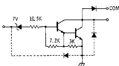
ULS-20X2* (Each Driver)
