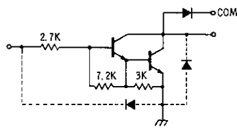
ULS-28X3* (Each Driver)
