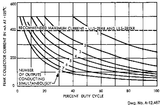
PEAK COLLECTOR CURRENT AS A FUNCTION OF DUTY CYCLE AT +125°C
