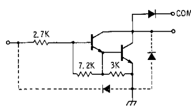
ULS-20X3* (Each Driver)
