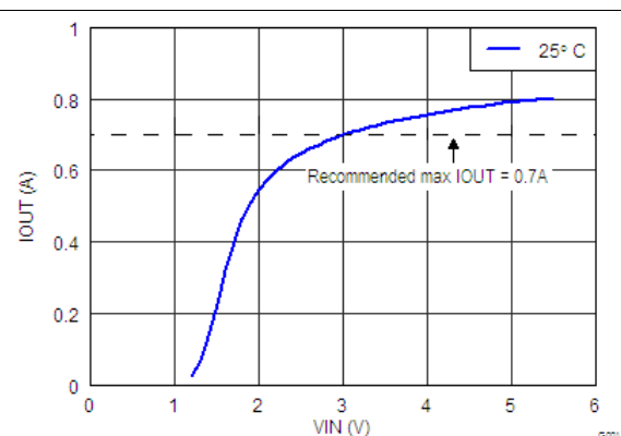
Figure 2. Load Current, 7-Channels in Parallel at V_{OL} = 0.6\text{ V}
