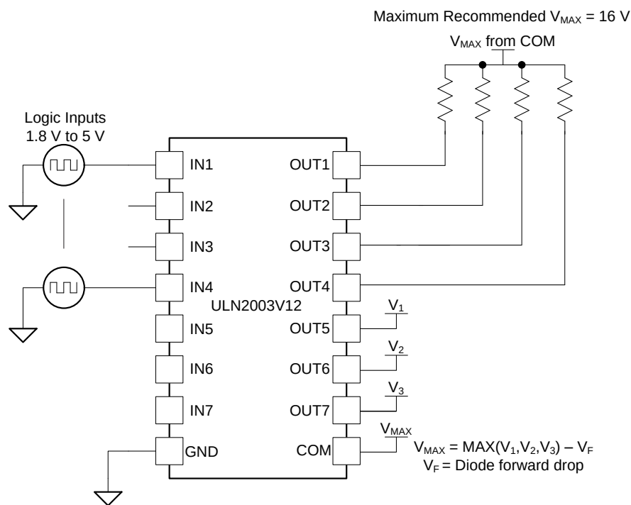
Figure 7. ULN2003V12 as a Maximum Supply Selector
