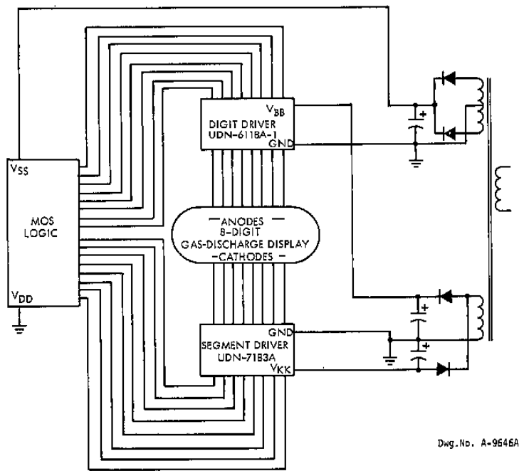
TYPICAL APPLICATION
