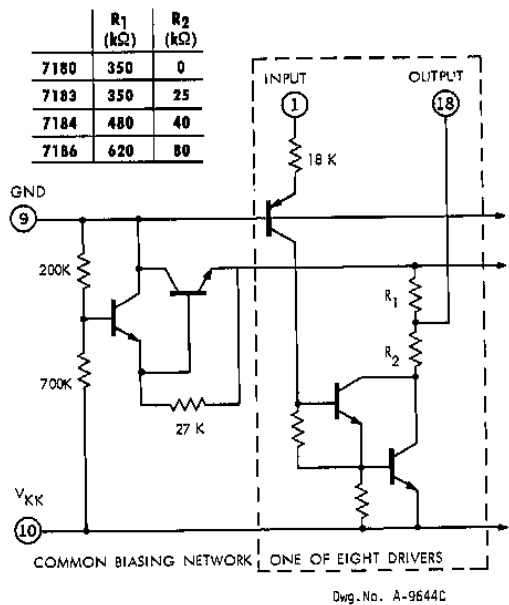
PARTIAL SCHEMATIC
