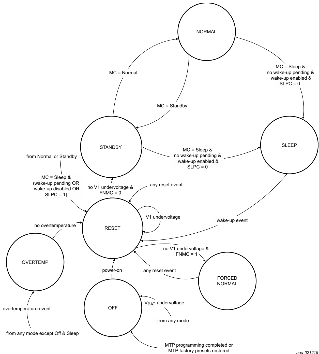
Fig 3. UJA1169L system controller state diagram
