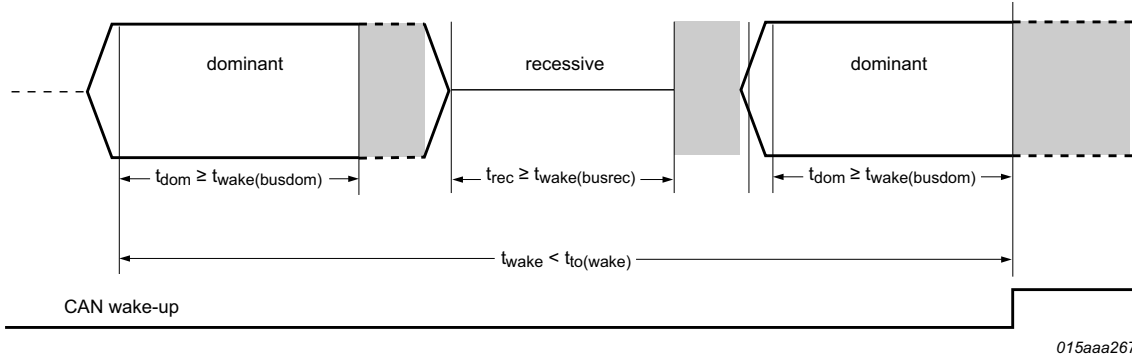
Fig 9. CAN wake-up timing
