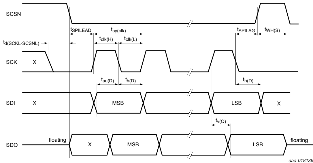
Fig 18. SPI timing diagram
