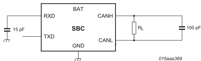
Fig 18. Timing test circuit for CAN transceiver
