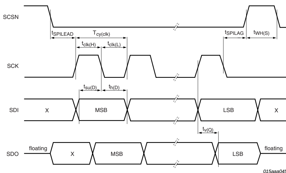
Fig 17. SPI timing diagram
