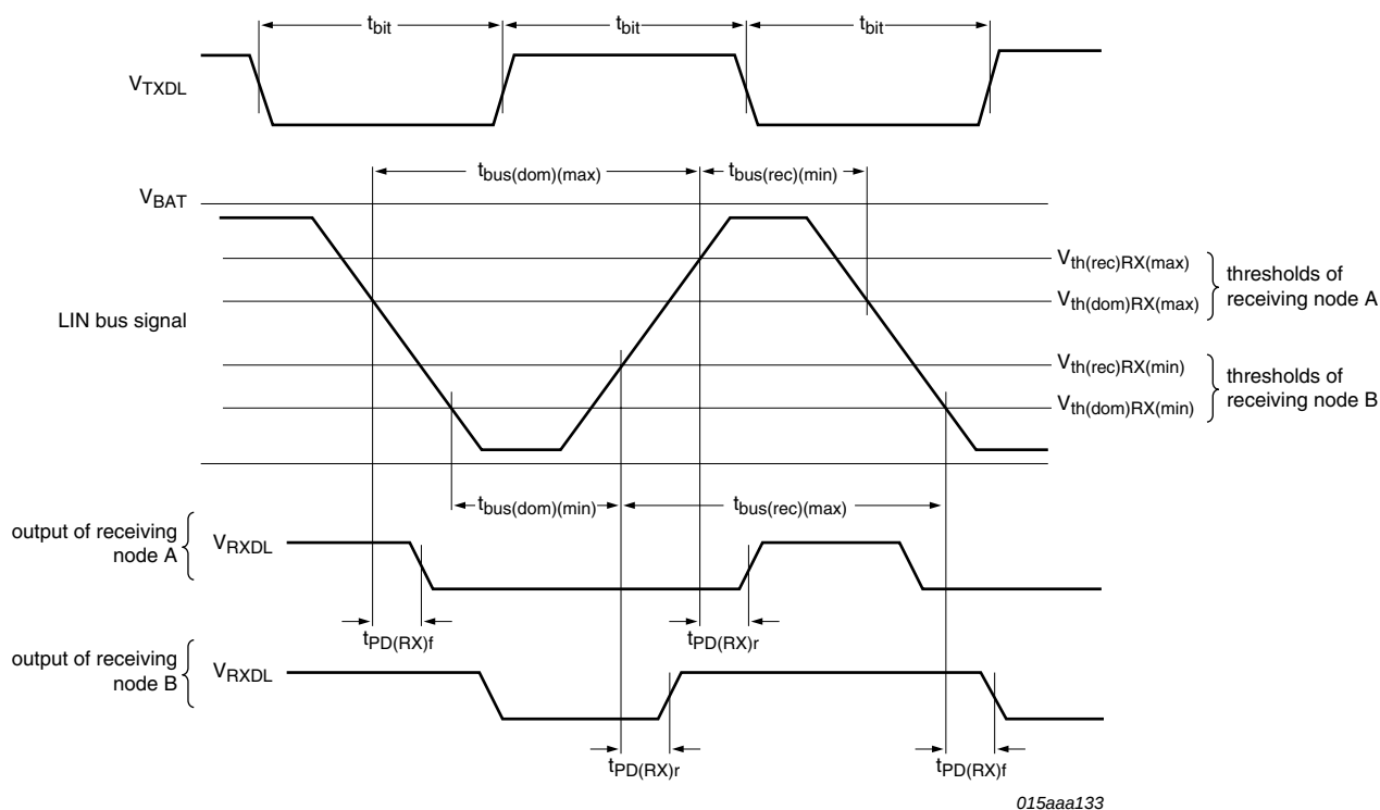
Fig 14. LIN transceiver timing diagram
